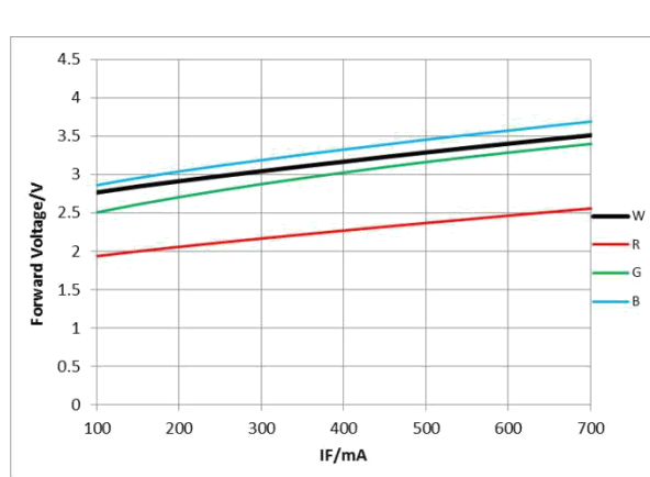
Fig 4. Forward Current vs. Forward Voltage, Ta = 25°C
