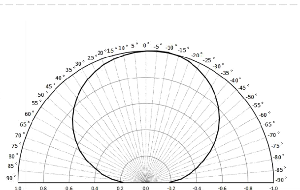
Fig 2. Viewing Angle Distribution, Ta = 25°C
