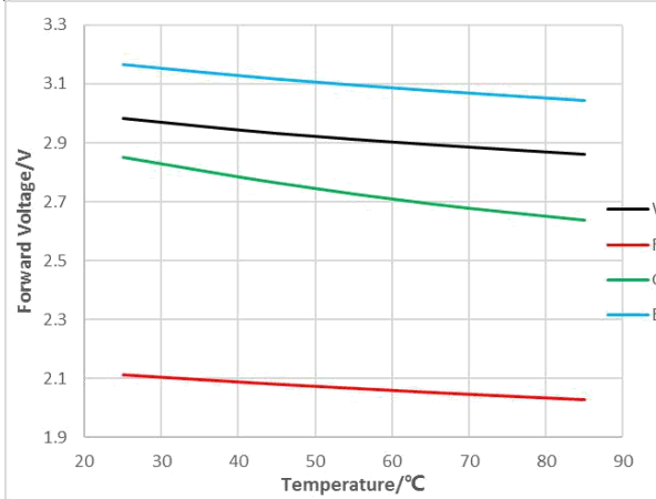
Fig 6. Ambient Temperature vs. Relative Forward Voltage (IF=350mA)
