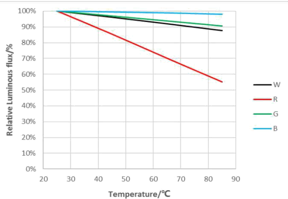
Fig 5. Ambient Temperature vs. Relative Luminous flux (IF=350mA)
