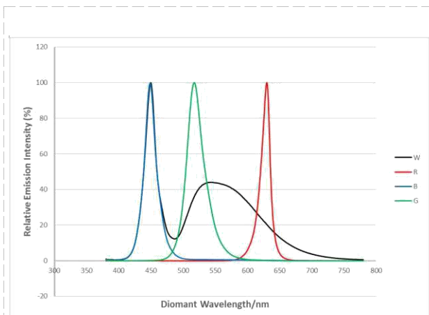
Fig 1. Color Spectrum, Ta = 25°C
