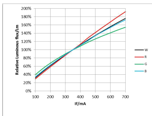
Fig 3. Forward Current vs. Relative Intensity, Ta = 25°C
